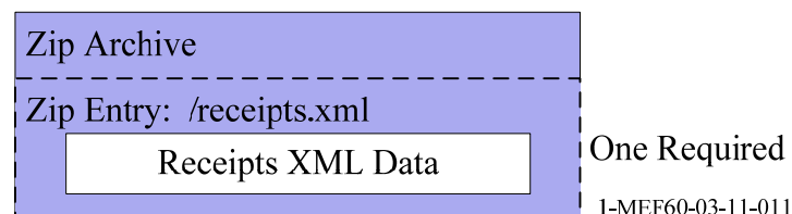
Figure 1-8. Receipts Structure
