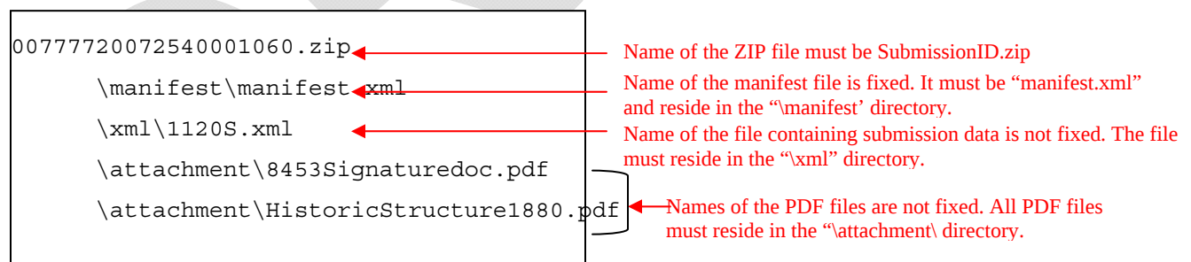
Figure 2-2: Sample IRS Submission Structure
