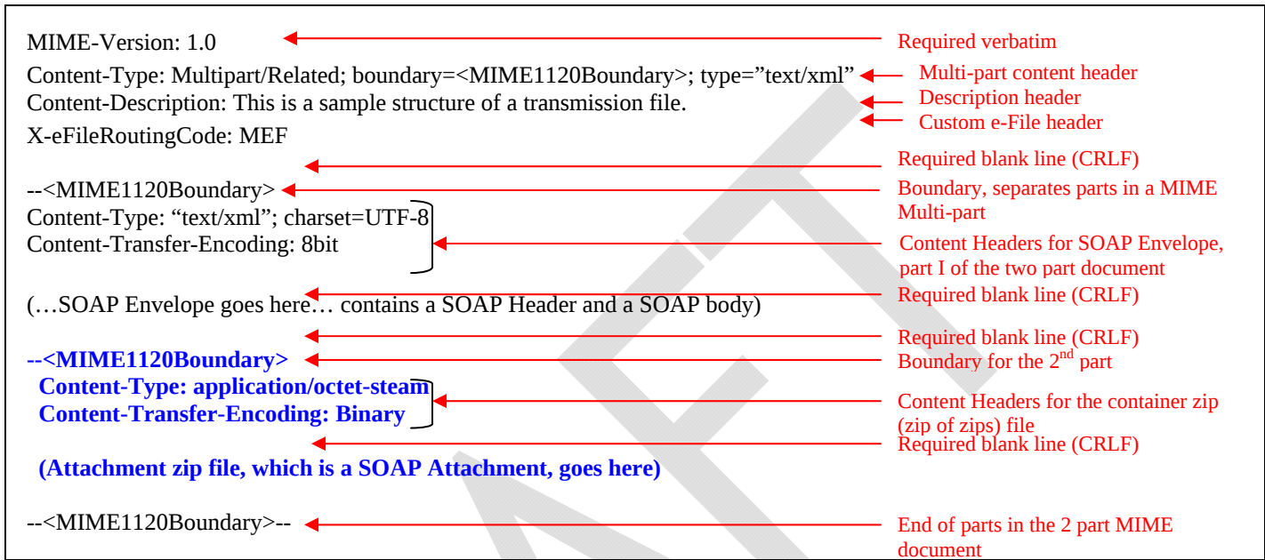
Figure 3–3: Sample Transmission File Submitted to IFA
