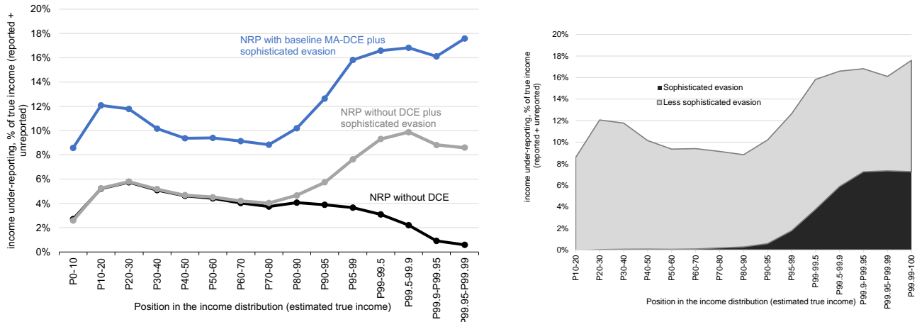
(a) Unreported Income (% True Income) Using Macro Allocated DCE (b) Composition of Unreported Income Using Macro Allocated DCE
